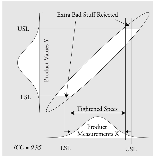
Figure 12: Specifications Tightened by Two Probable Errors
