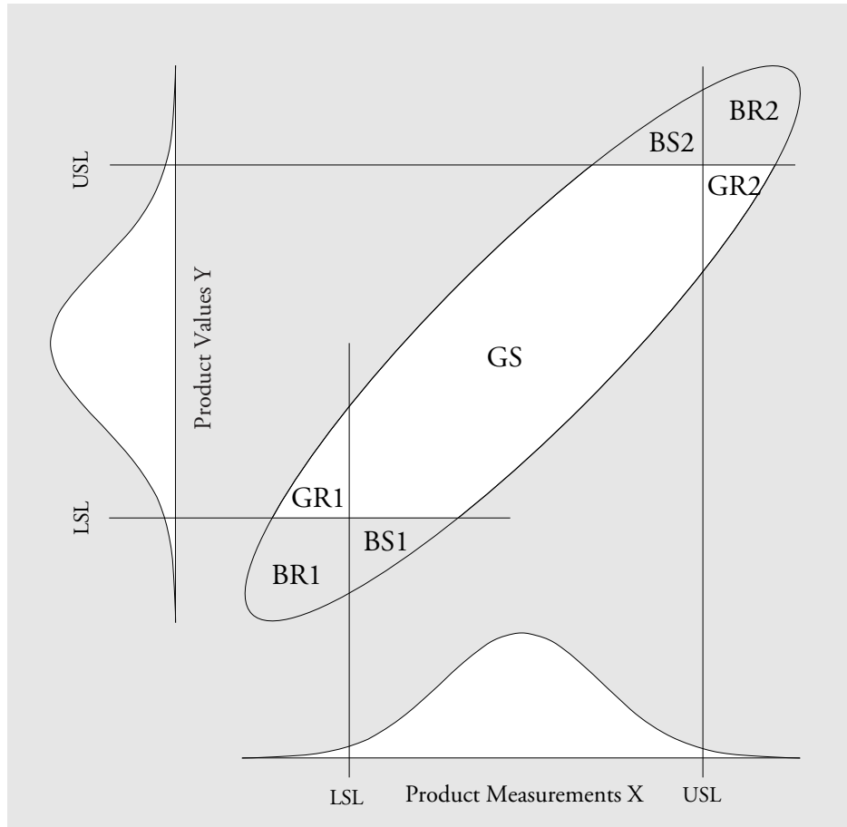
Figure 6: The Four Outcomes of 100% Inspection
