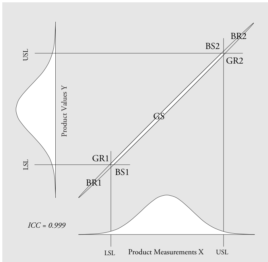
Figure 8: One Way to Avoid Misclassifications with 100% Inspection
