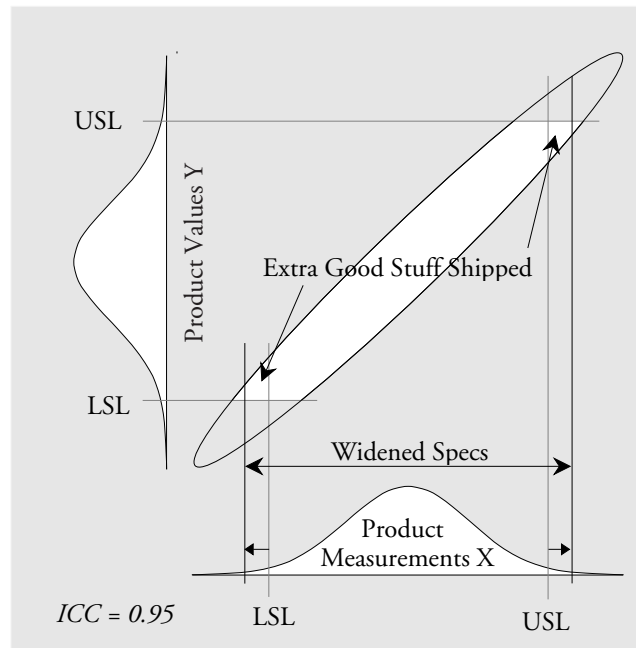
Figure 10: Specifications Widened by Two Probable Errors
