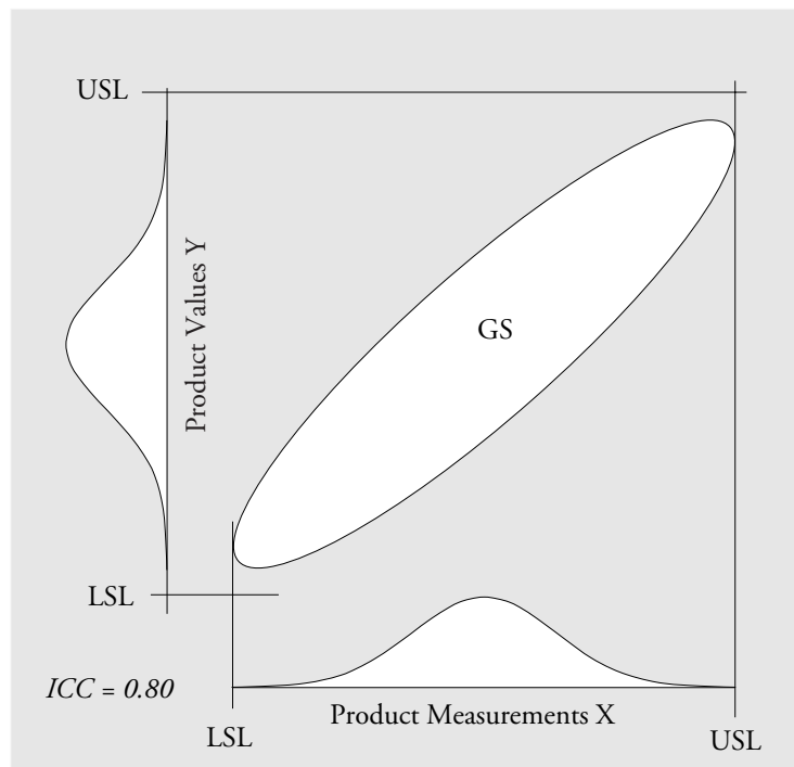
Figure 9: The Only Sure Way to Avoid Shipping Nonconforming Product
